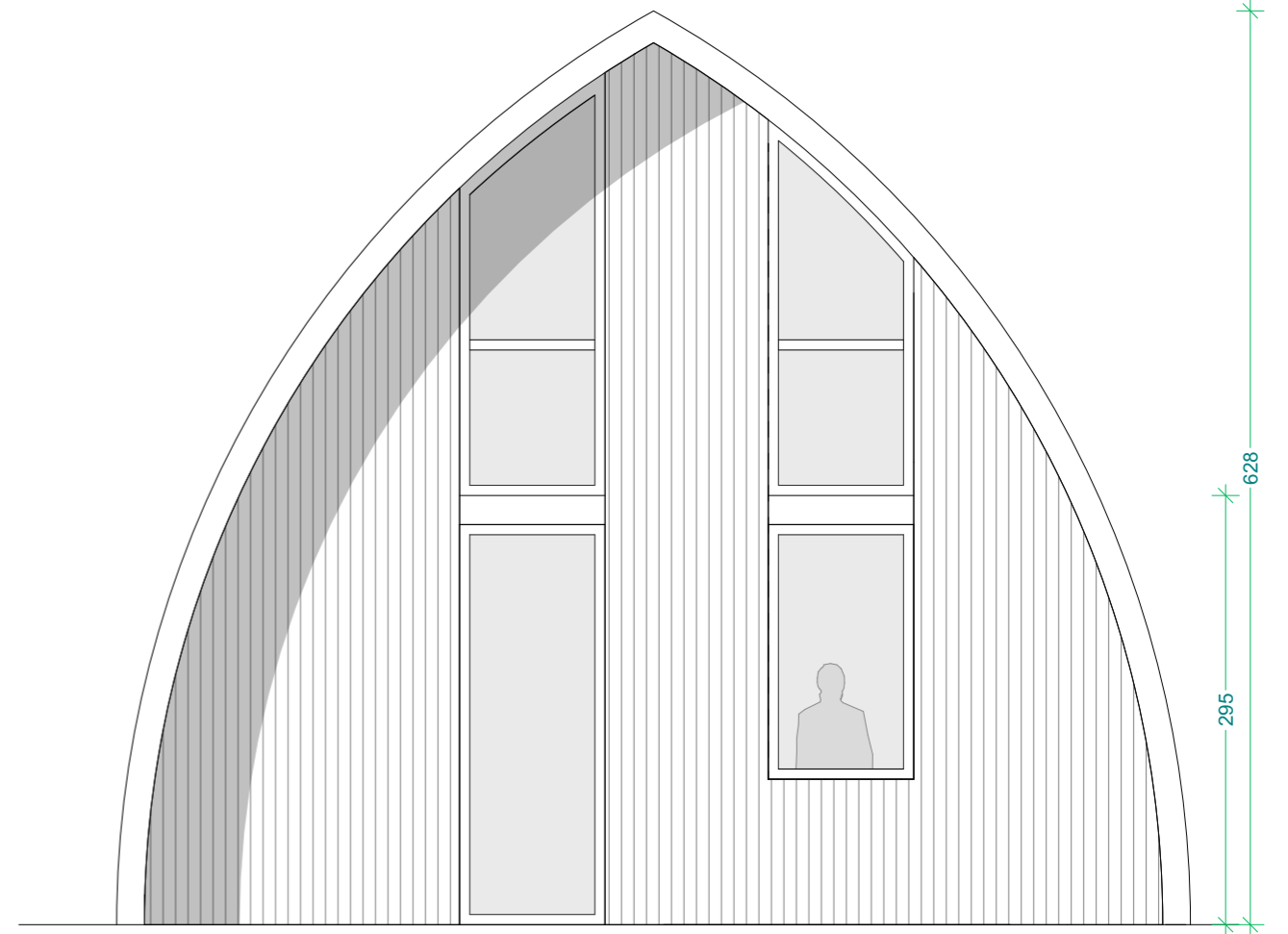
FACADE "NORD"
