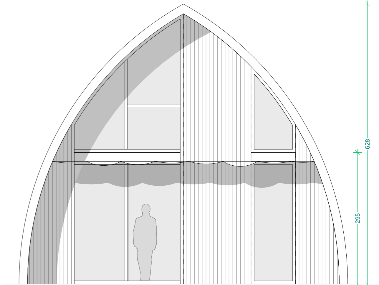
FACADE "NORD"
